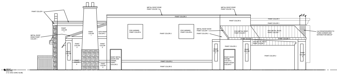
SOUTH ELEVATION 1/4" = 1'-0"
