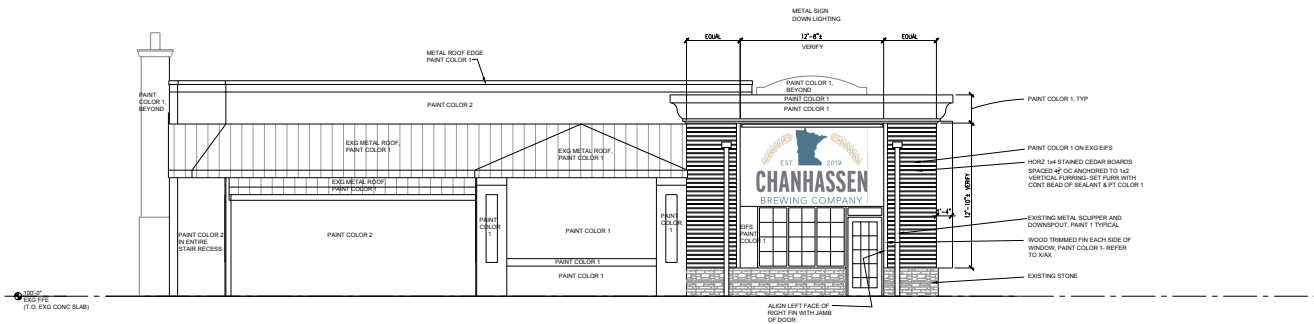
EAST ELEVATION 1/4" = 1'-0"
